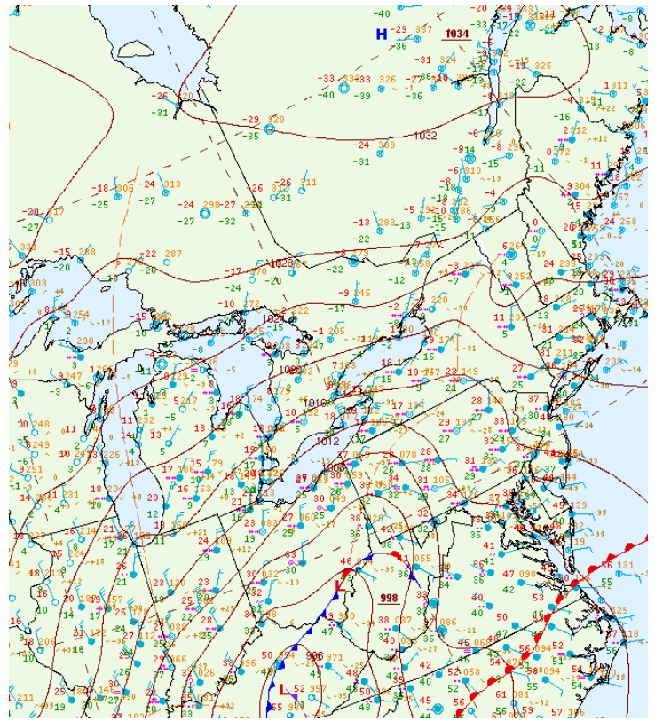
Fig. 2. Surface analysis 00 UTC on 20 January 2019.
