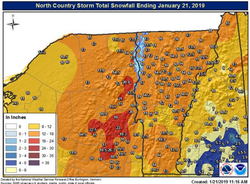
Fig. 1 (above). Storm total snowfall amounts 19-21 January 2019.
